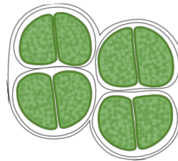
Chroococcus
