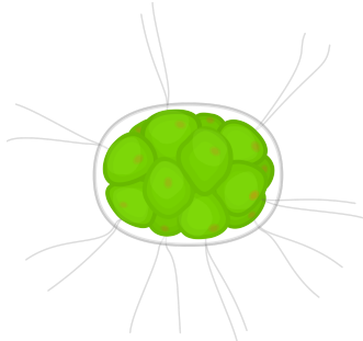
Pandorina
