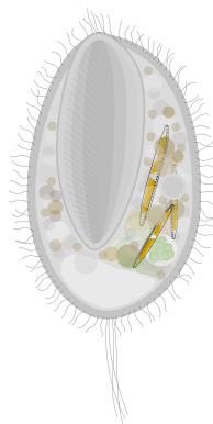
Lembadion
