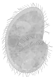
Colpoda
