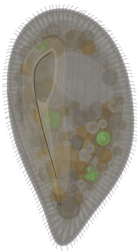
Frontonia atra
