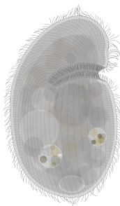
Plagiopyla
