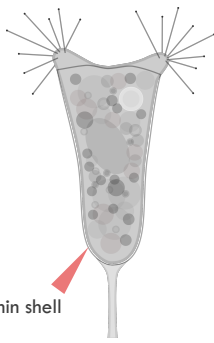
Acineta
