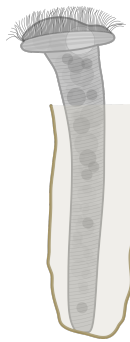
Vaginicola
