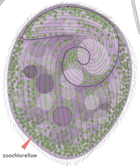
Stentor amethystinus
